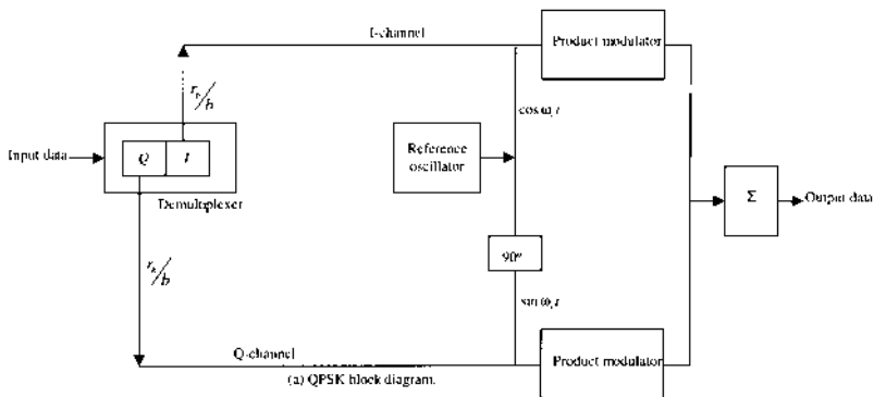
FIGURE 3.3 QPSK modulator.
