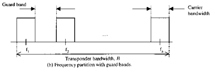
FIGURE 5.2 Principle of FDMA system: (a) multiple access by frequency; (b) frequency partition with guard bands.
