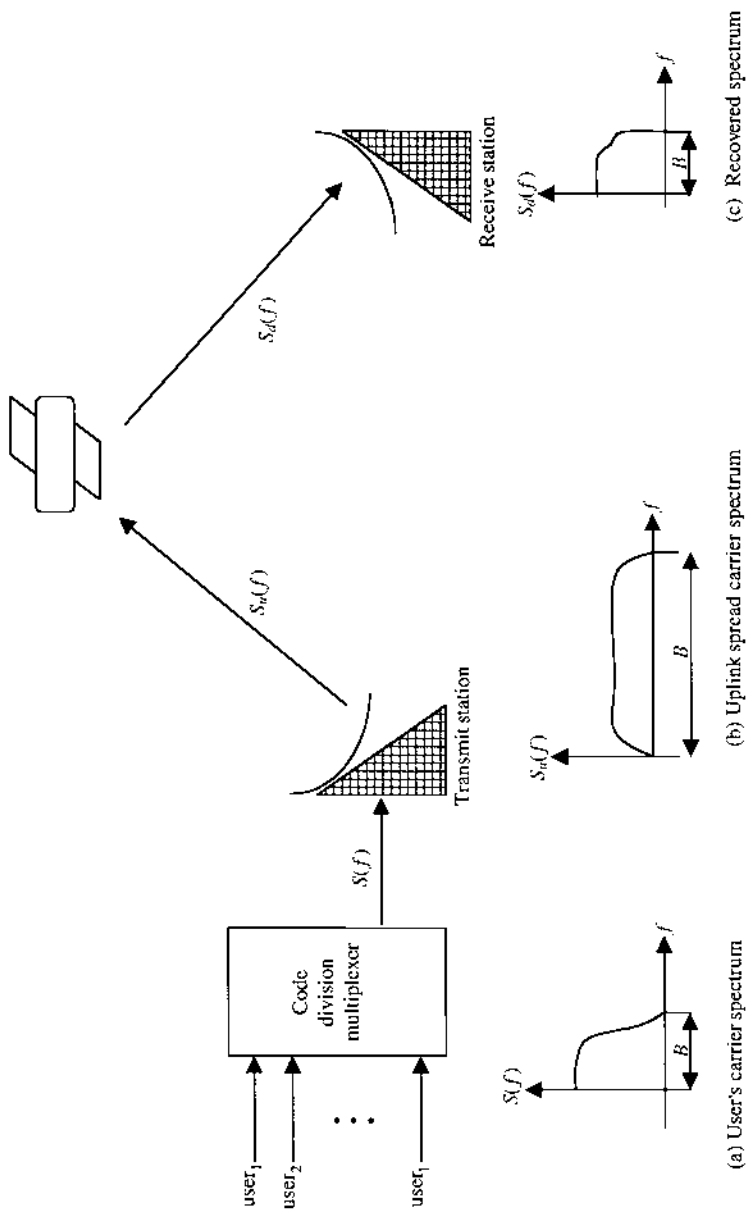
FIGURE 5.7 CDMA system: (a) user's carrier spectrum; (b) uplink spread carrier spectrum; (c) recovered spectrum.
